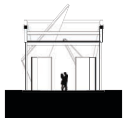
SECTION BB 1/8" = 1'
